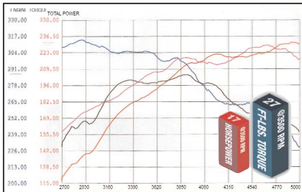
Dyno Results
